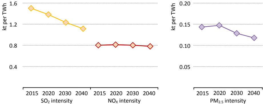
Figure 9.2 ▶ Emissions intensity in the power sector by pollutant in Southeast Asia in the New Policies Scenario
